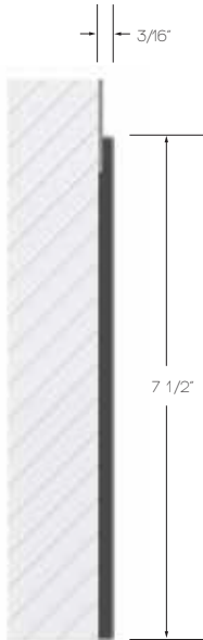
1 BASE - LARGE VWBL-**-144 3/16" x 7 1/2" x 144"L
