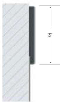
6 TOP RAIL VWR-**-144 1/4" x 3" x 144"L (also for finished ends)
